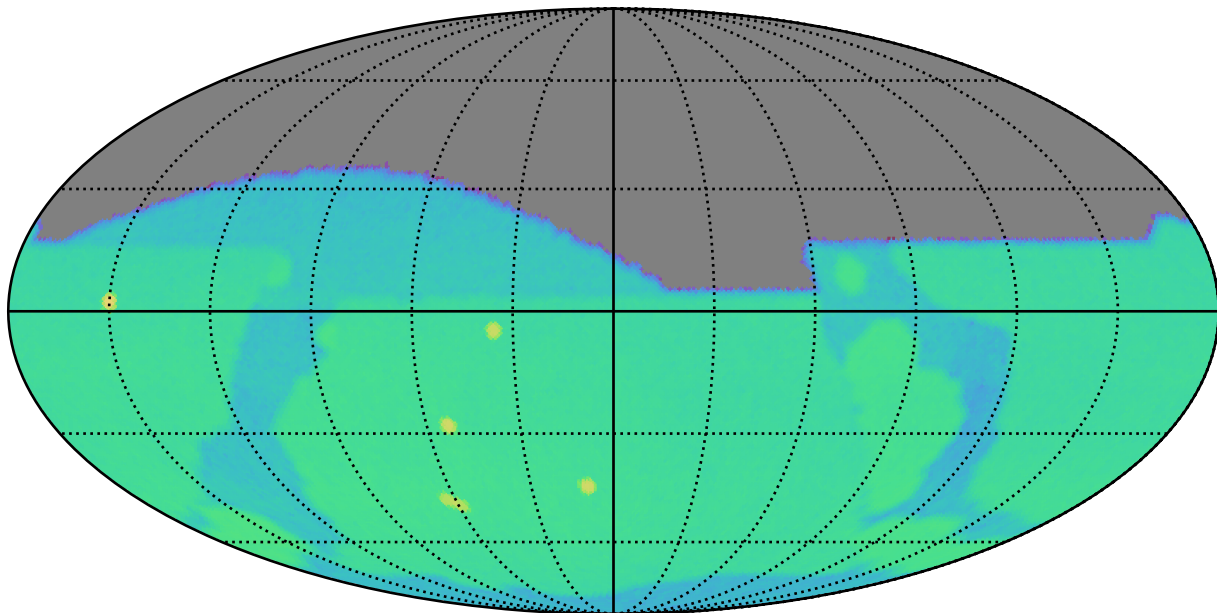
noroll_mjdp60_v3.4_10yrs g: SurfaceBrightLimit
