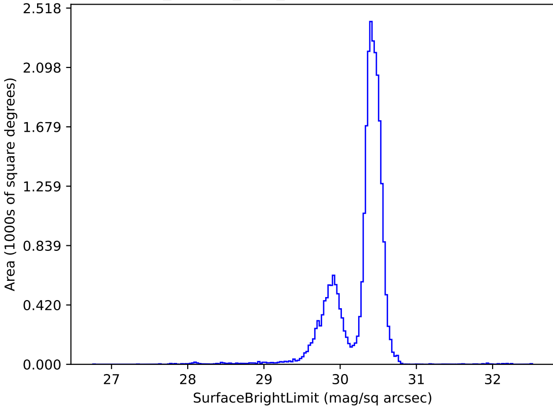
noroll_mjdp60_v3.4_10yrs g: SurfaceBrightLimit
