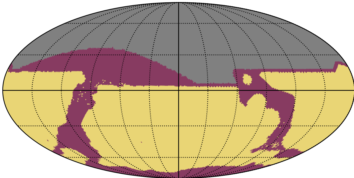
noroll_mjdp60_v3.4_10yrs : RapidRevisits
