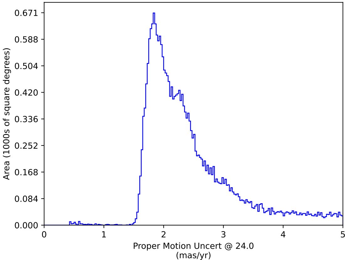
noroll_mjdp60_v3.4_10yrs : Proper Motion Uncert @ 24.0
