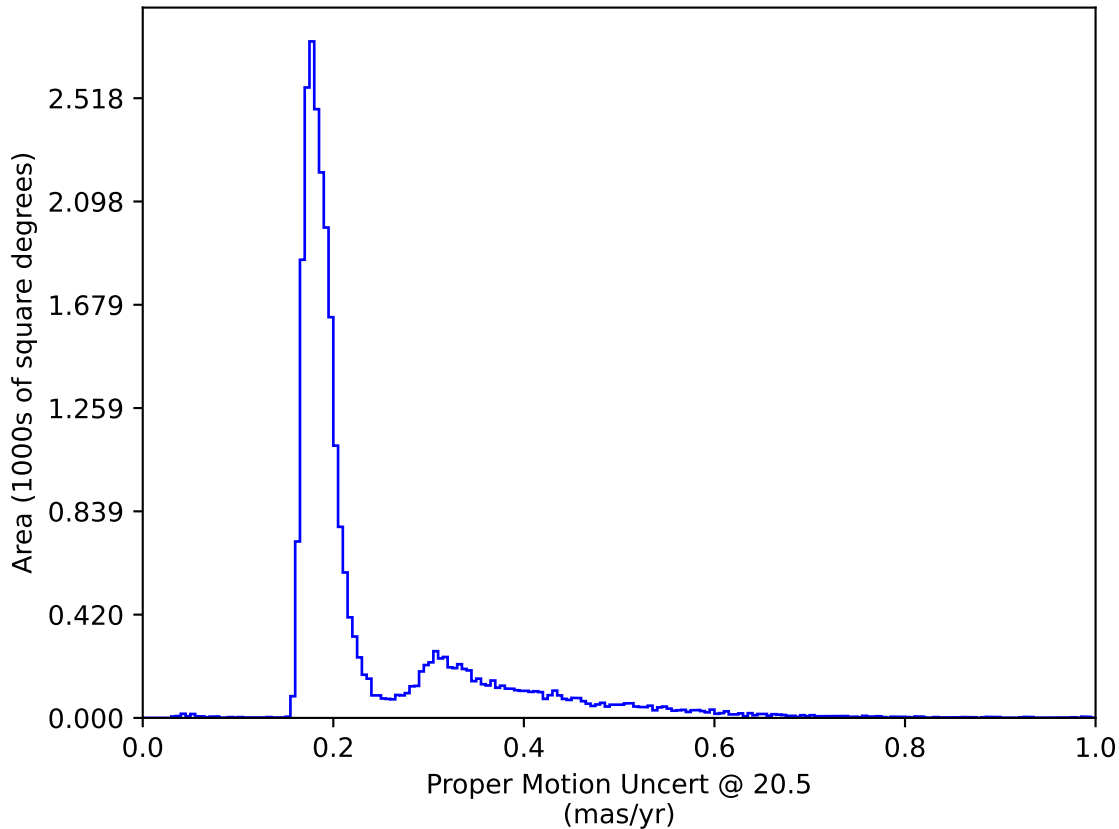
noroll_mjdp60_v3.4_10yrs : Proper Motion Uncert @ 20.5
