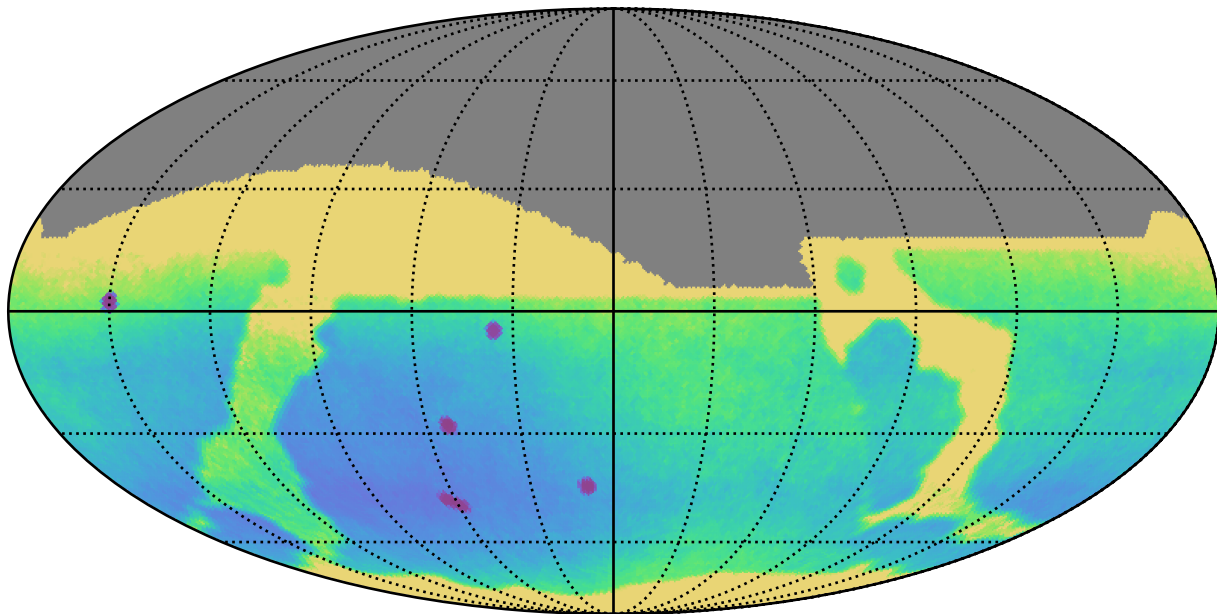
noroll_mjdp60_v3.4_10yrs : Parallax Uncert @ 24.0
