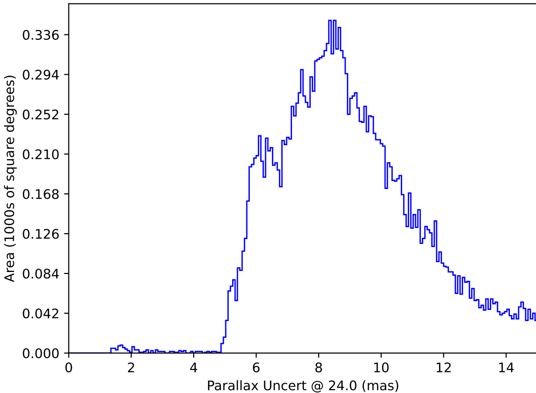
noroll_mjdp60_v3.4_10yrs : Parallax Uncert @ 24.0
