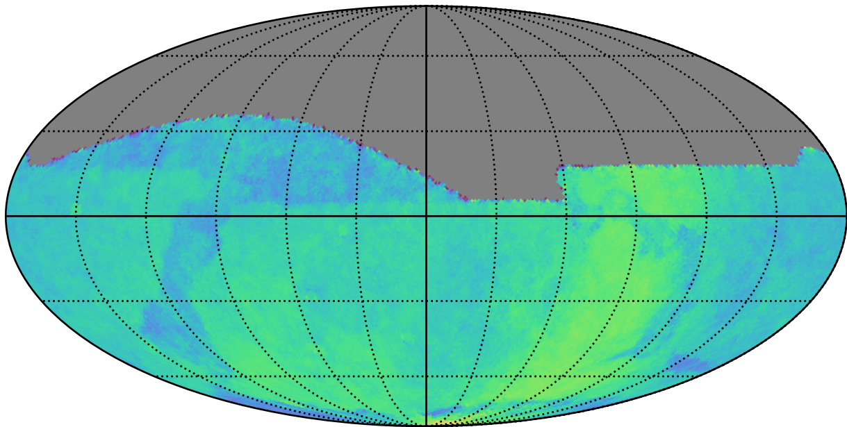
noroll_mjdp60_v3.4_10yrs : Parallax Coverage @ 24.0
