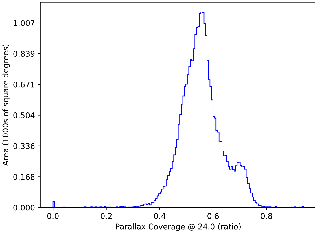
noroll_mjdp60_v3.4_10yrs : Parallax Coverage @ 24.0
