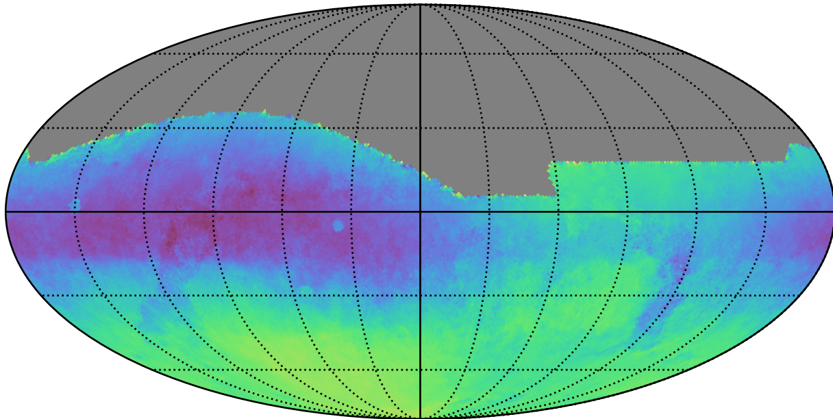
noroll_mjdp60_v3.4_10yrs : Parallax-DCR degeneracy @ 24.0
