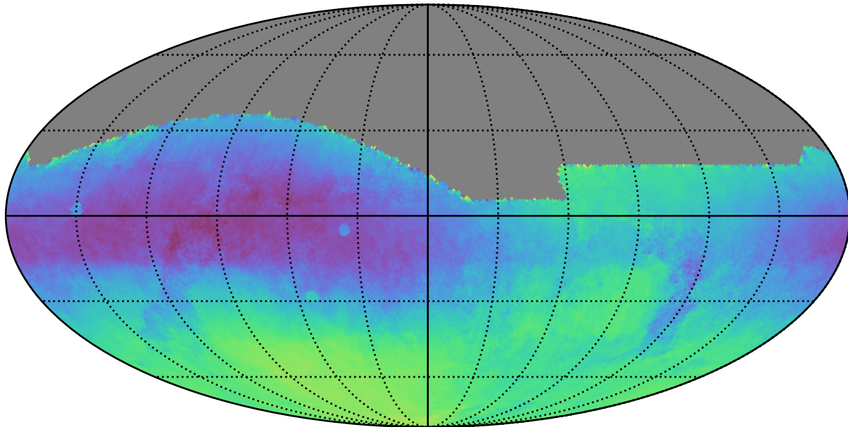
noroll_mjdp60_v3.4_10yrs : Parallax-DCR degeneracy @ 22.4
