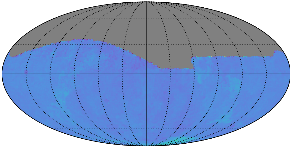
noroll_mjdp60_v3.4_10yrs : Normalized Proper Motion Uncert @ 24.0
