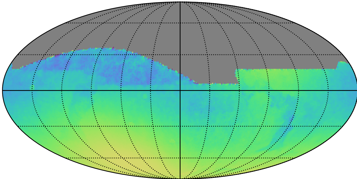
noroll_mjdp60_v3.4_10yrs : Normalized Parallax Uncert @ 22.4
