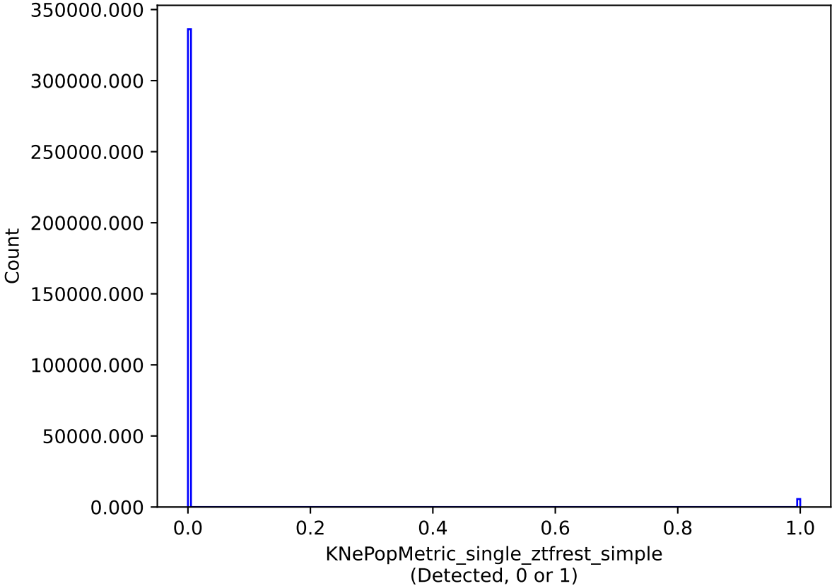
noroll_mjdp60_v3.4_10yrs single model: KNePopMetric_single_ztfrest_simple
