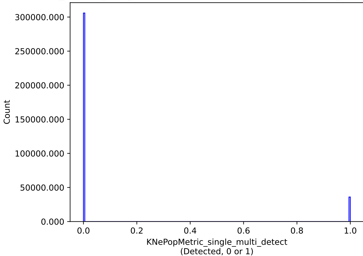
noroll_mjdp60_v3.4_10yrs single model: KNePopMetric_single_multi_detect
