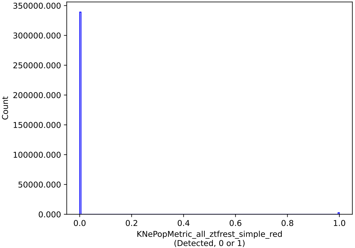
noroll_mjdp60_v3.4_10yrs all models: KNePopMetric_all_ztfrest_simple_red
