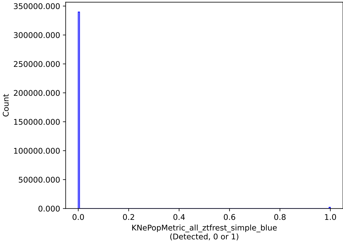
noroll_mjdp60_v3.4_10yrs all models: KNePopMetric_all_ztfrest_simple_blue
