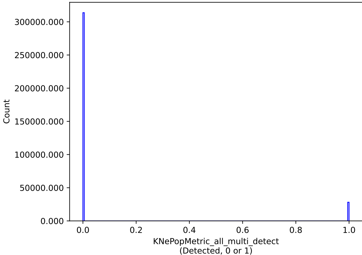
noroll_mjdp60_v3.4_10yrs all models: KNePopMetric_all_multi_detect
