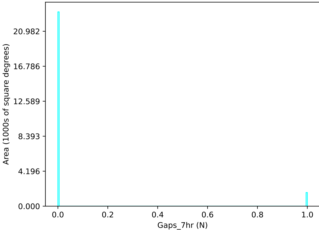
noroll_mjdp60_v3.4_10yrs u band: Gaps_7hr
