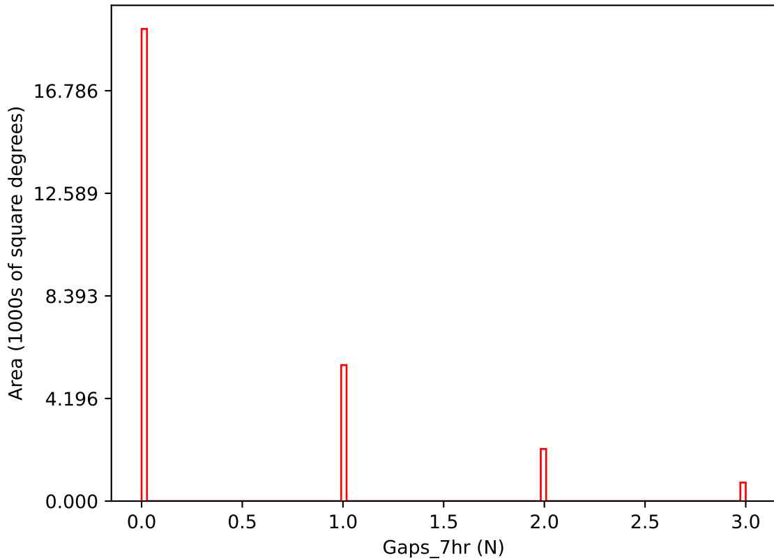
noroll_mjdp60_v3.4_10yrs i band: Gaps_7hr
