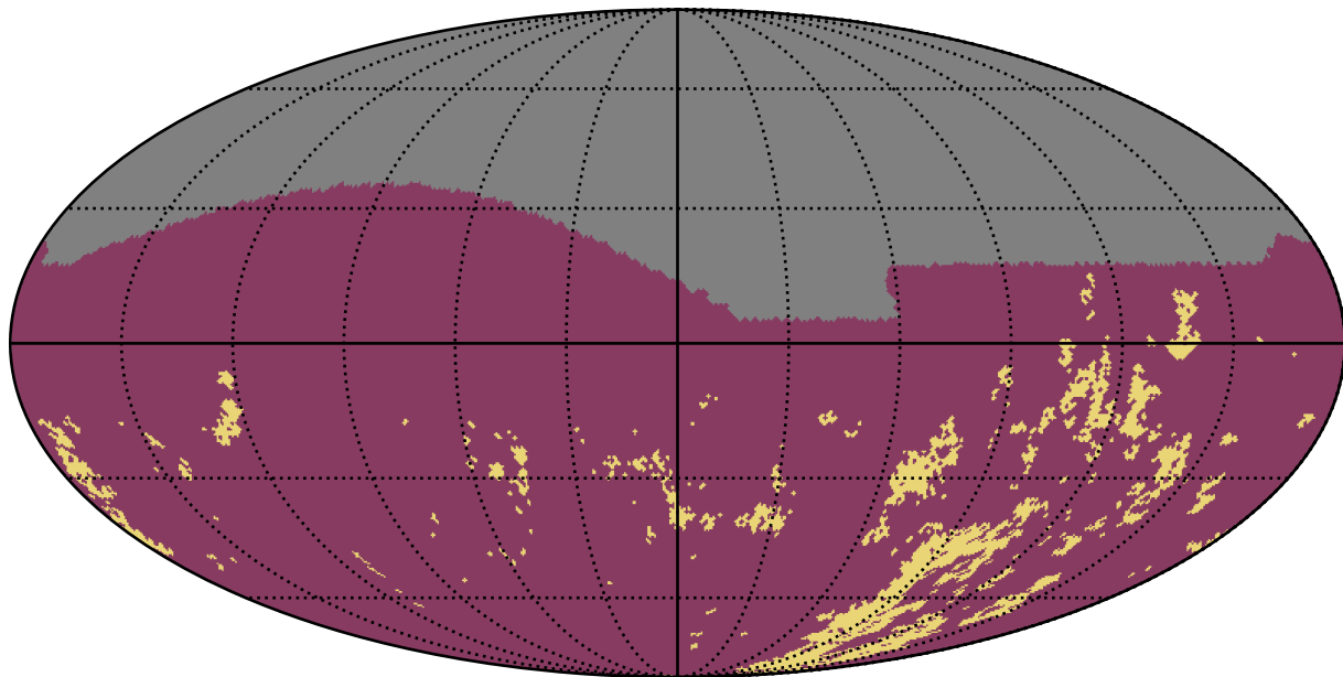
noroll_mjdp60_v3.4_10yrs g band: Gaps_7hr
