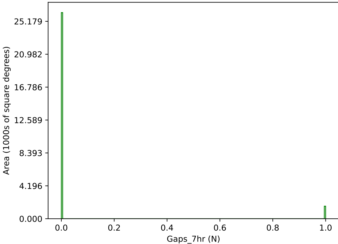
noroll_mjdp60_v3.4_10yrs g band: Gaps_7hr
