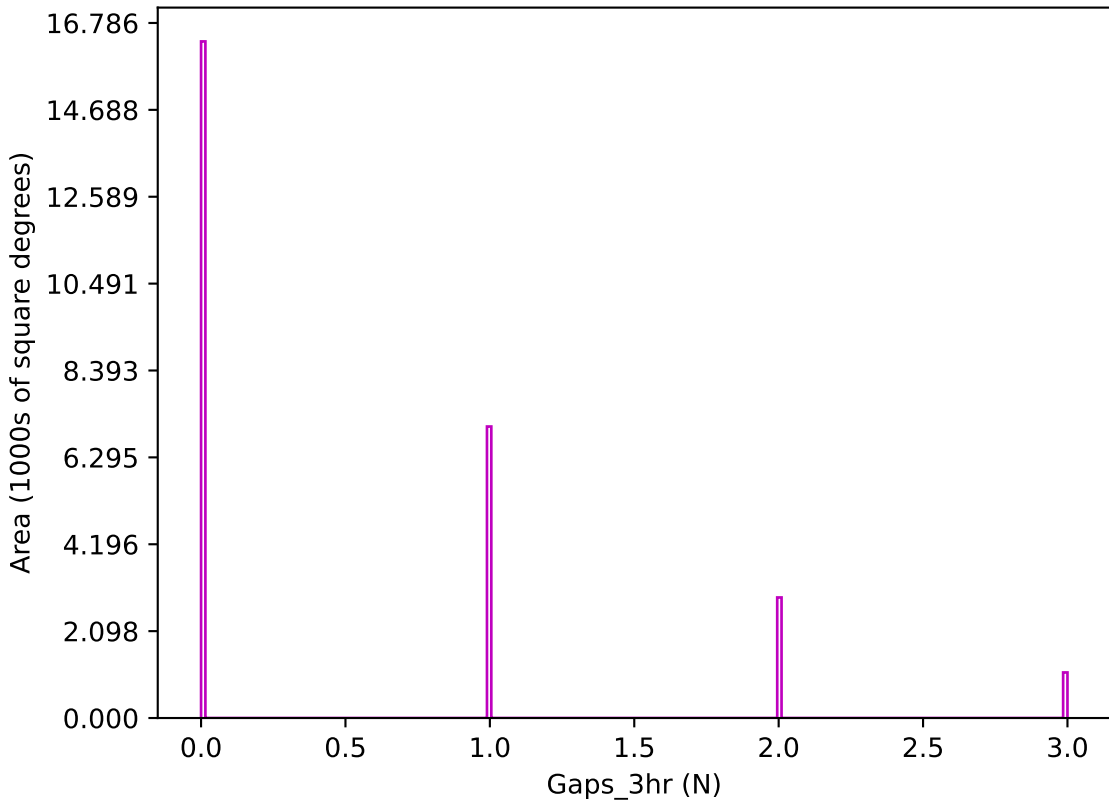
noroll_mjdp60_v3.4_10yrs z band: Gaps_3hr
