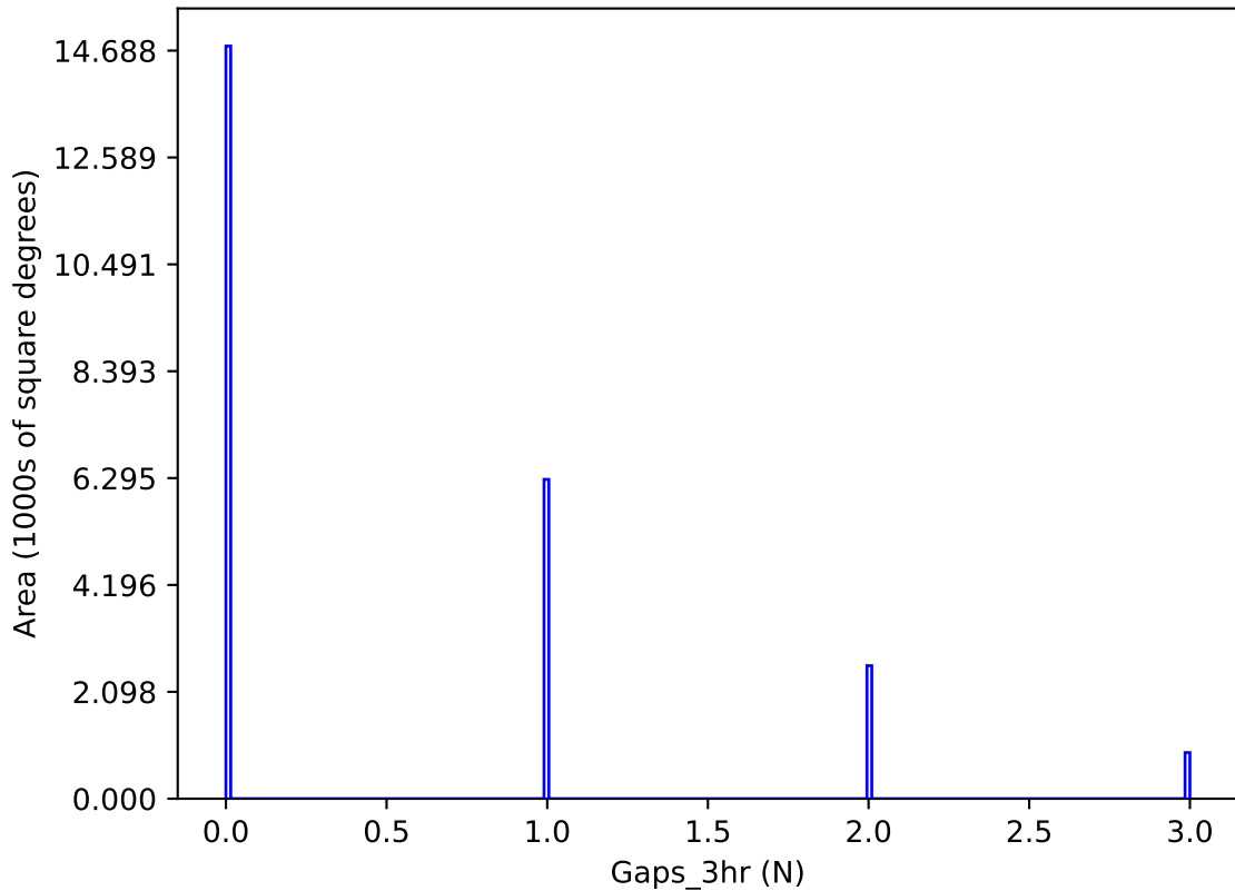
noroll_mjdp60_v3.4_10yrs y band: Gaps_3hr
