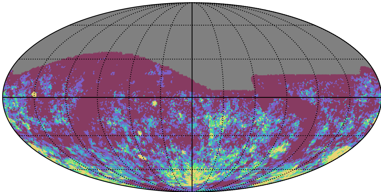
noroll_mjdp60_v3.4_10yrs i band: Gaps_3hr
