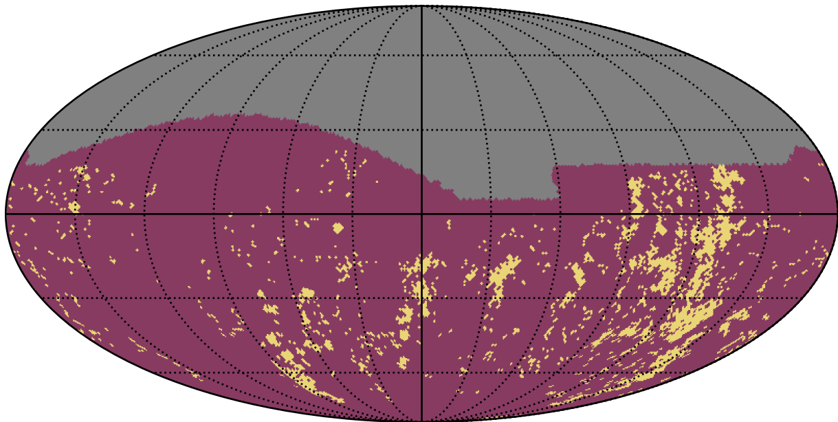
noroll_mjdp60_v3.4_10yrs g band: Gaps_3hr
