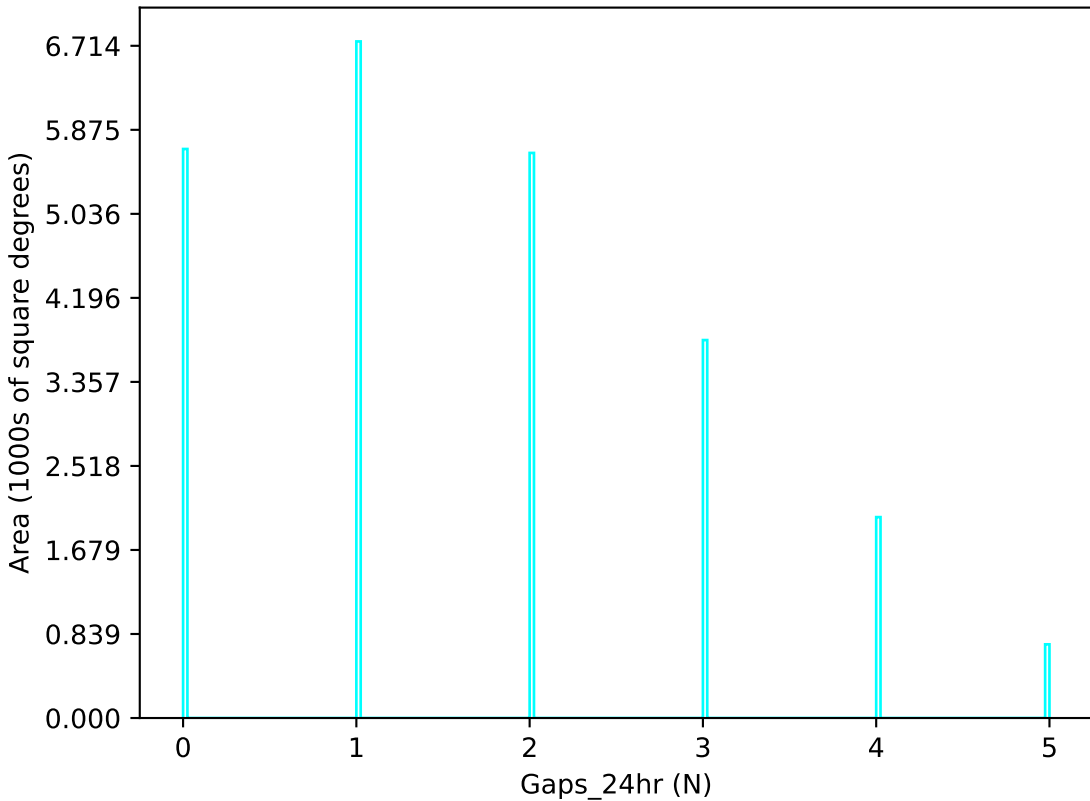
noroll_mjdp60_v3.4_10yrs u band: Gaps_24hr
