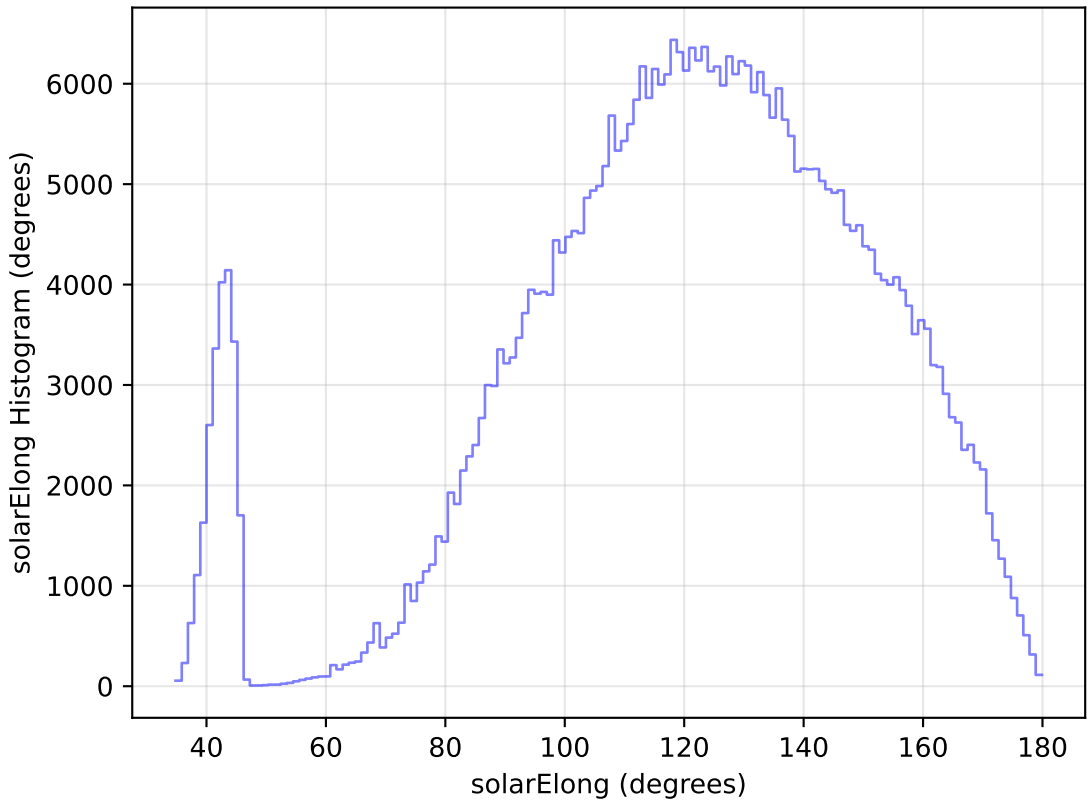
noroll_mjdp60_v3.4_10yrs WFD z band: solarElong Histogram
