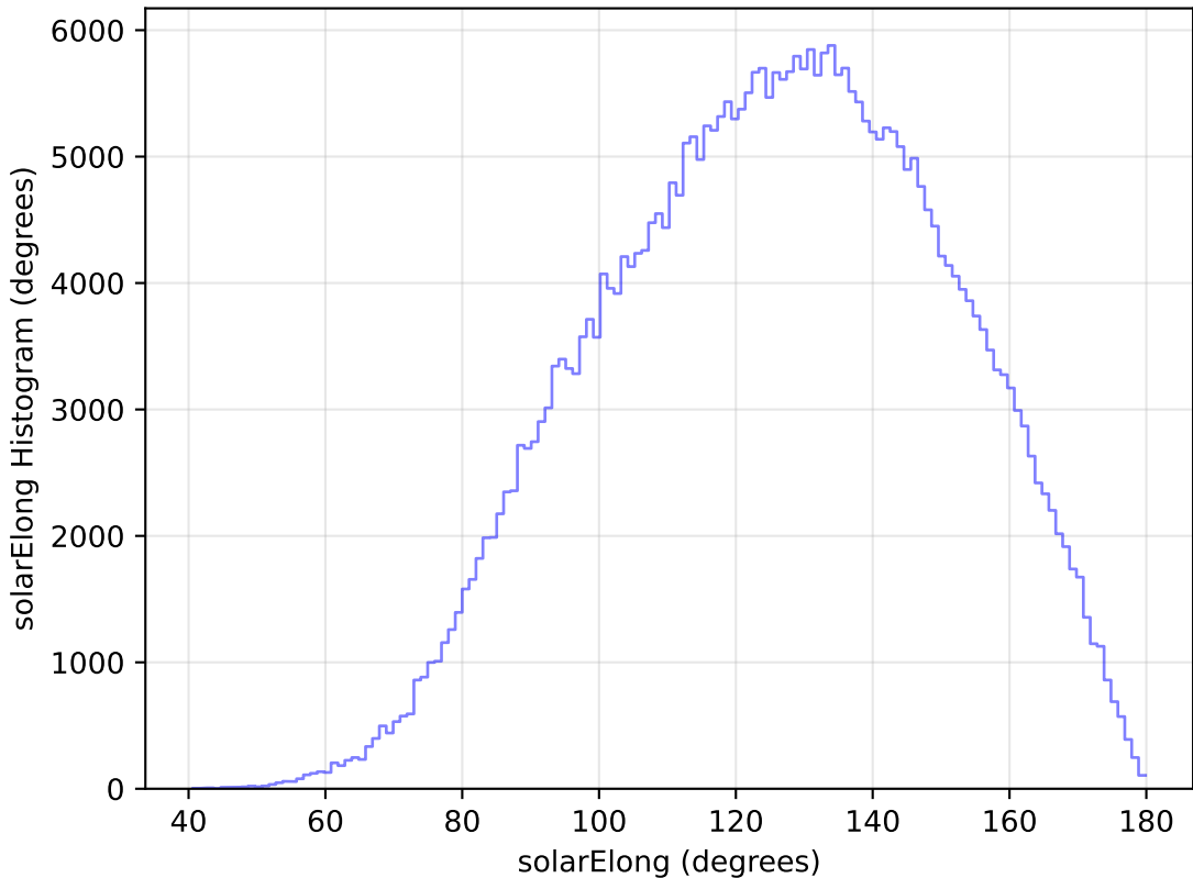
noroll_mjdp60_v3.4_10yrs WFD y band: solarElong Histogram
