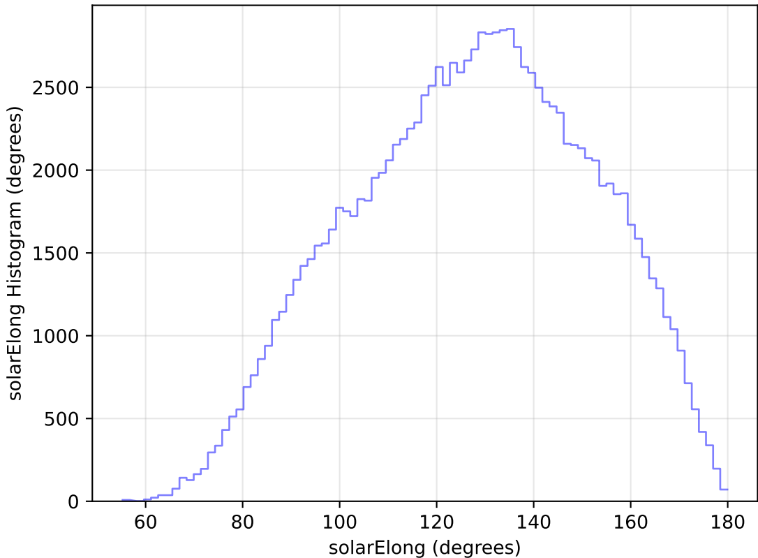
noroll_mjdp60_v3.4_10yrs WFD u band: solarElong Histogram
