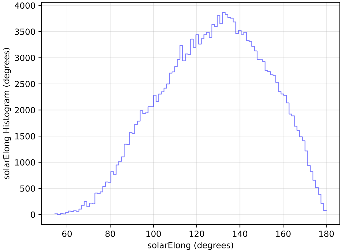
noroll_mjdp60_v3.4_10yrs WFD g band: solarElong Histogram
