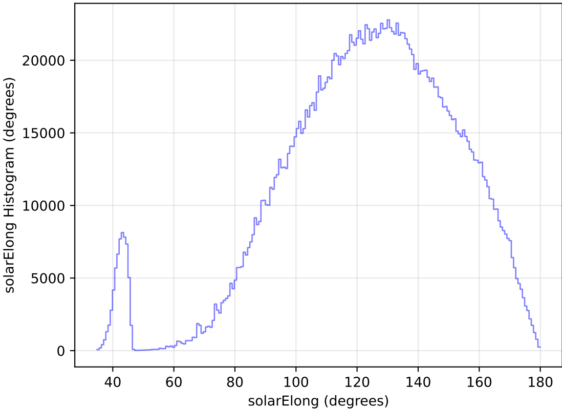
noroll_mjdp60_v3.4_10yrs WFD all bands: solarElong Histogram
