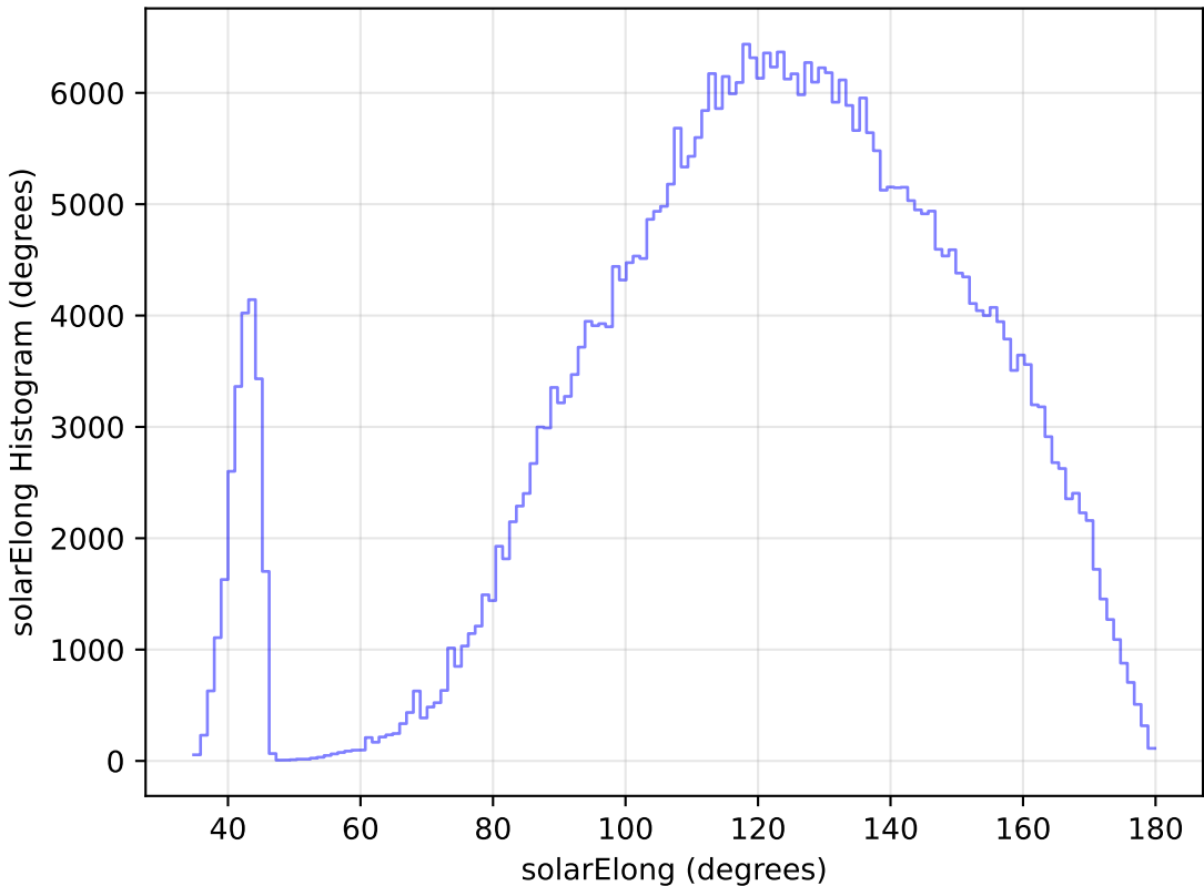
noroll_mjdp60_v3.4_10yrs All sky z band: solarElong Histogram
