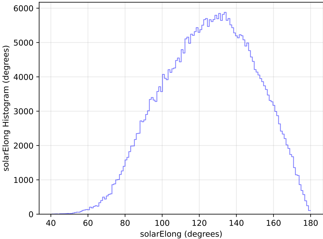
noroll_mjdp60_v3.4_10yrs All sky y band: solarElong Histogram
