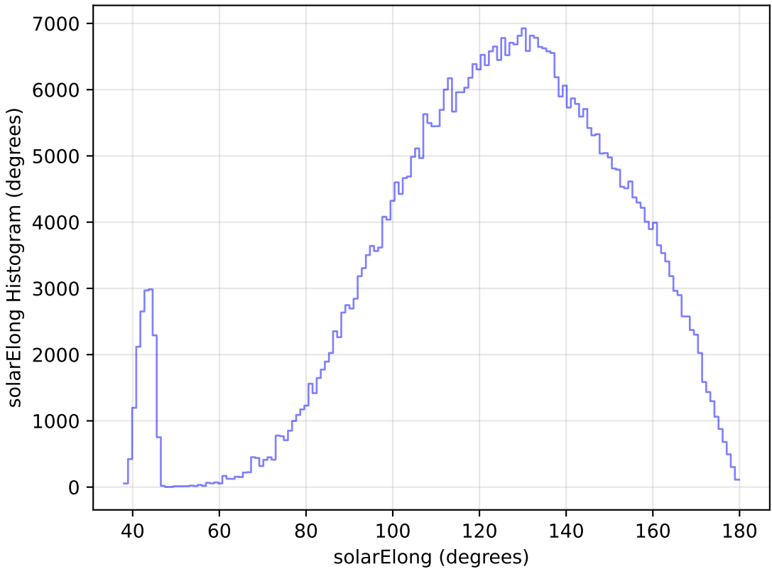
noroll_mjdp60_v3.4_10yrs All sky r band: solarElong Histogram
