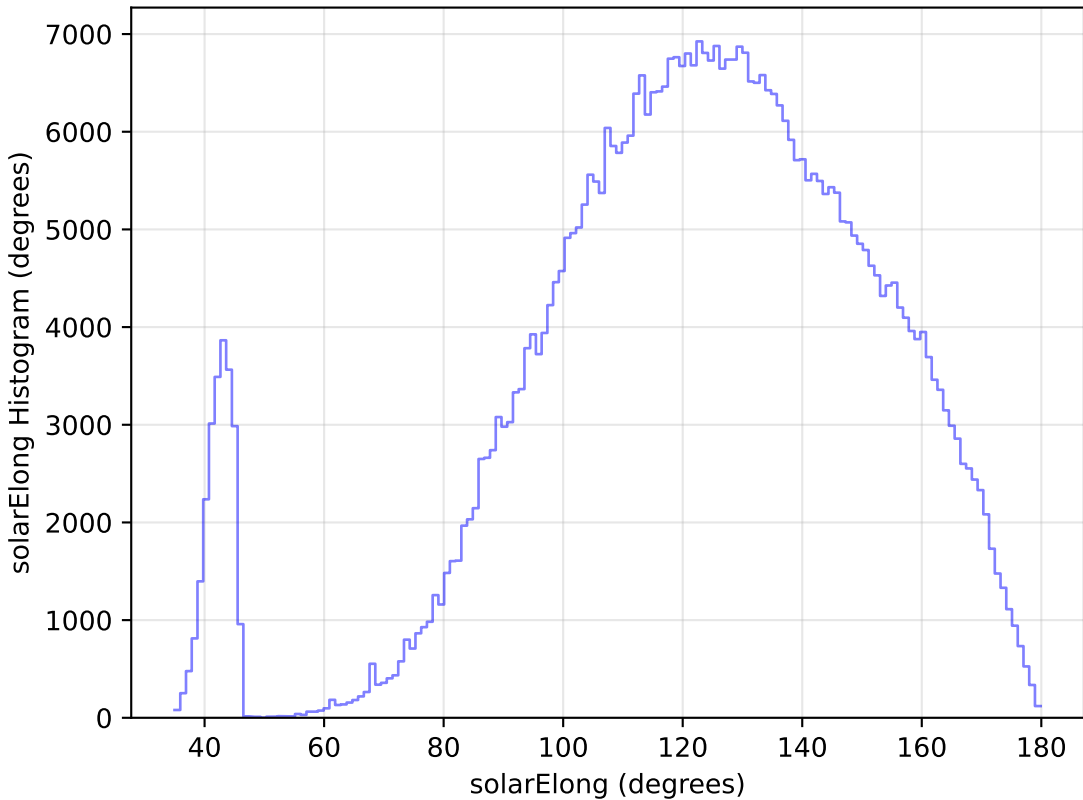
noroll_mjdp60_v3.4_10yrs All sky i band: solarElong Histogram
