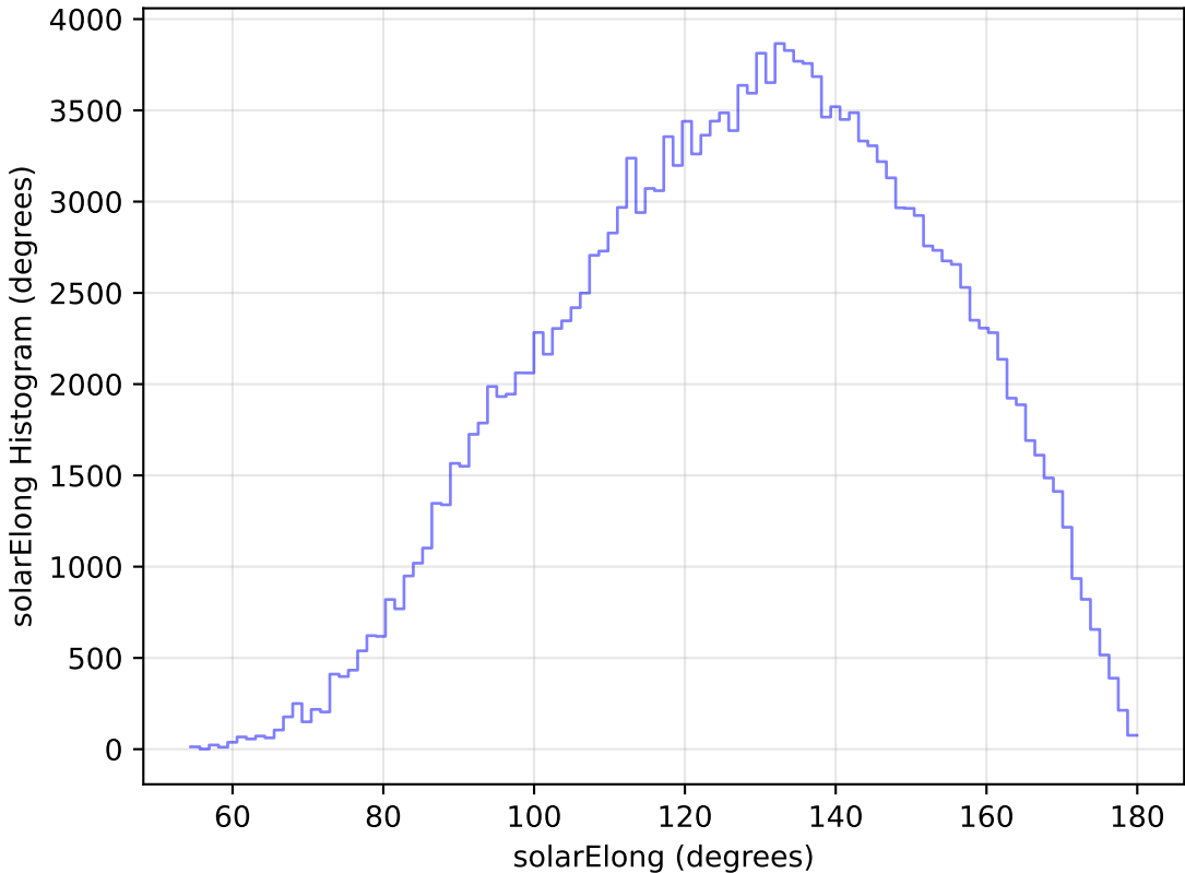
noroll_mjdp60_v3.4_10yrs All sky g band: solarElong Histogram
