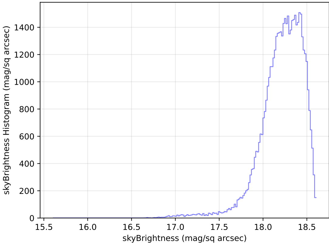
noroll_mjdp60_v3.4_10yrs Yr 1 y band: skyBrightness Histogram
