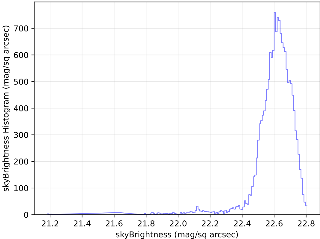
noroll_mjdp60_v3.4_10yrs Yr 1 u band: skyBrightness Histogram
