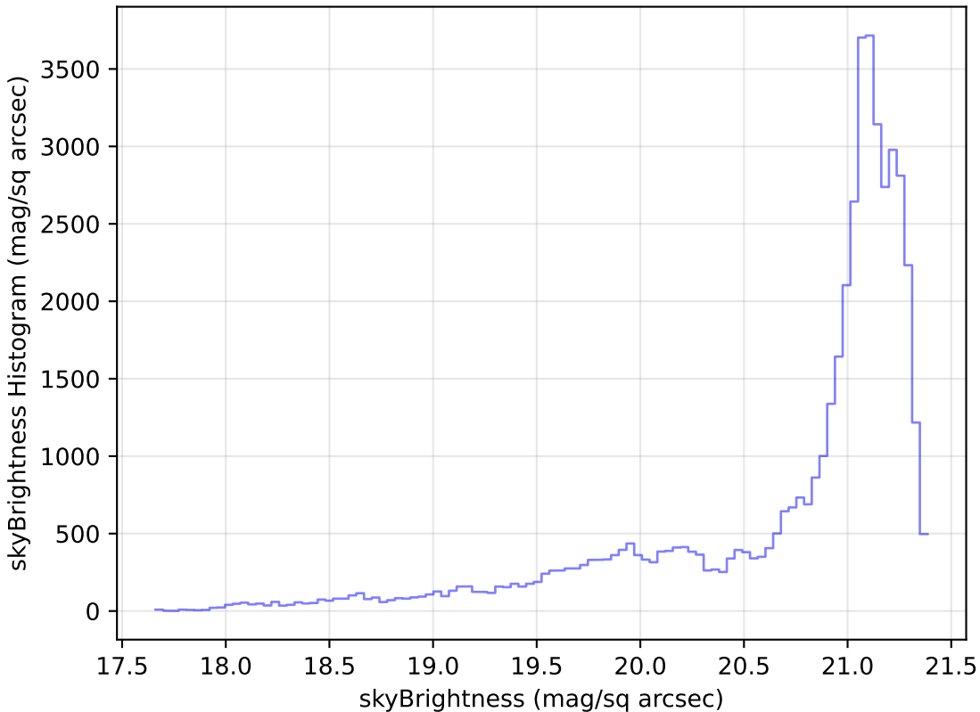
noroll_mjdp60_v3.4_10yrs Yr 1 r band: skyBrightness Histogram
