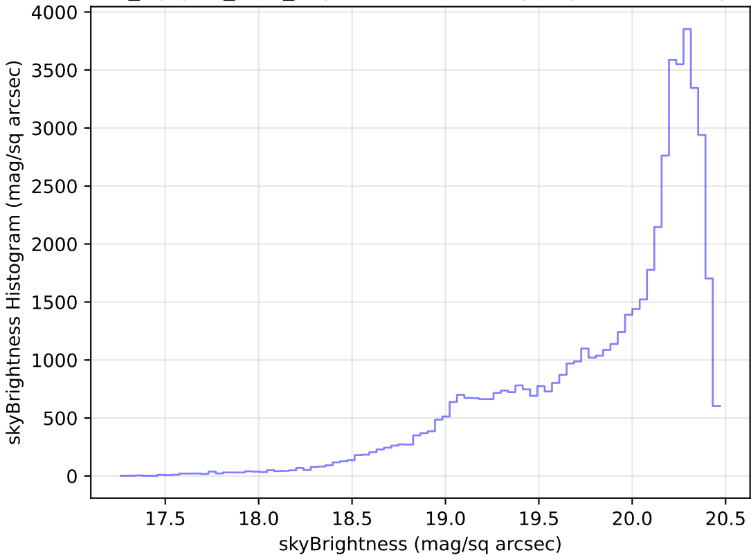
noroll_mjdp60_v3.4_10yrs Yr 1 i band: skyBrightness Histogram
