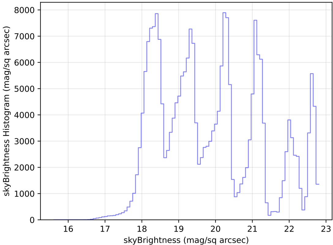
noroll_mjdp60_v3.4_10yrs Yr 1 all bands: skyBrightness Histogram
