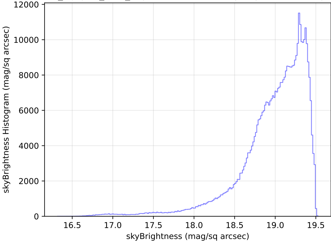
noroll_mjdp60_v3.4_10yrs WFD z band: skyBrightness Histogram
