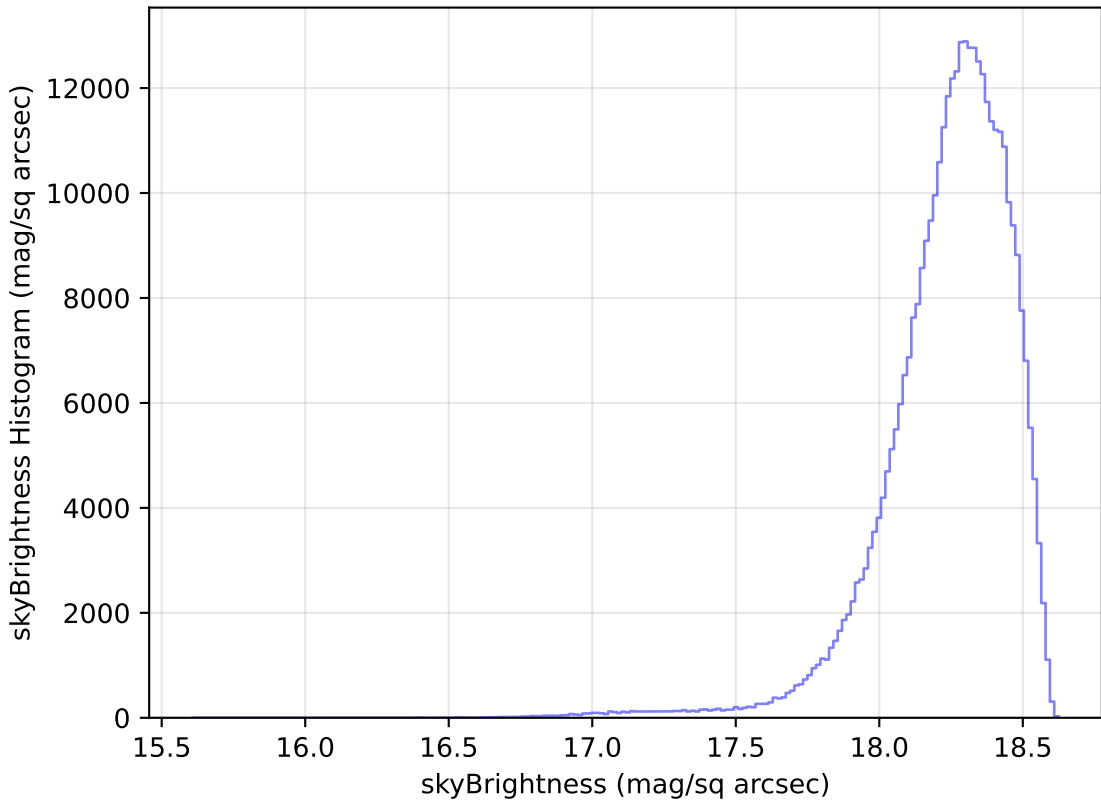
noroll_mjdp60_v3.4_10yrs WFD y band: skyBrightness Histogram
