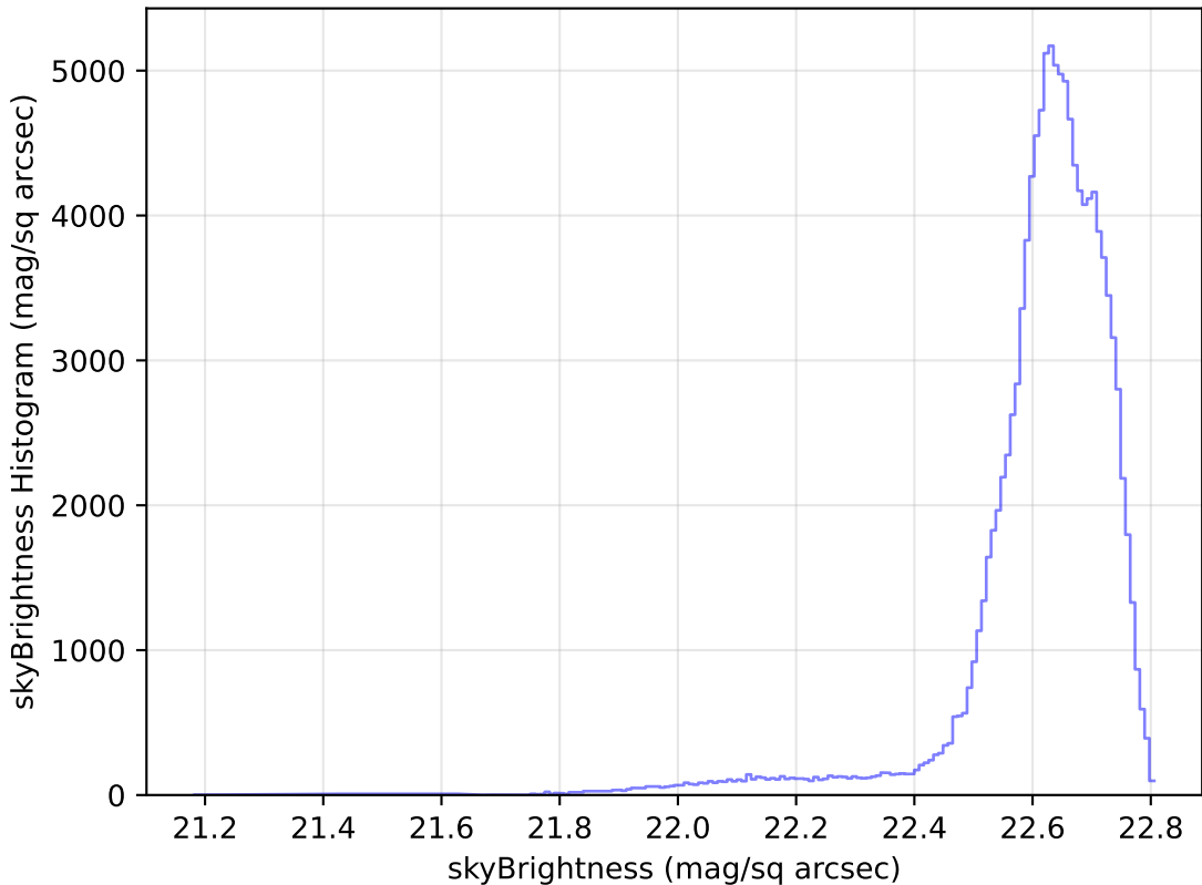
noroll_mjdp60_v3.4_10yrs WFD u band: skyBrightness Histogram
