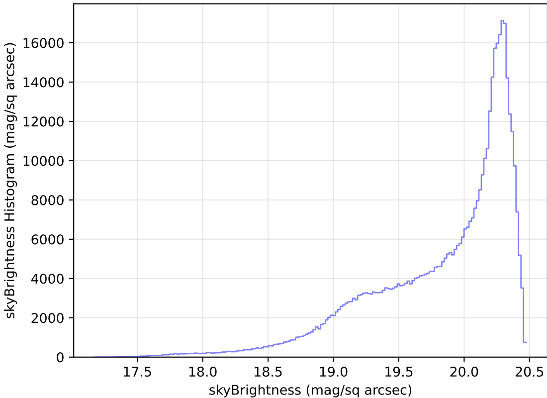
noroll_mjdp60_v3.4_10yrs WFD i band: skyBrightness Histogram
