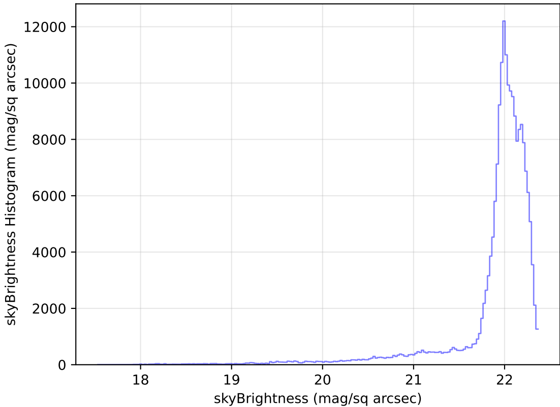
noroll_mjdp60_v3.4_10yrs WFD g band: skyBrightness Histogram
