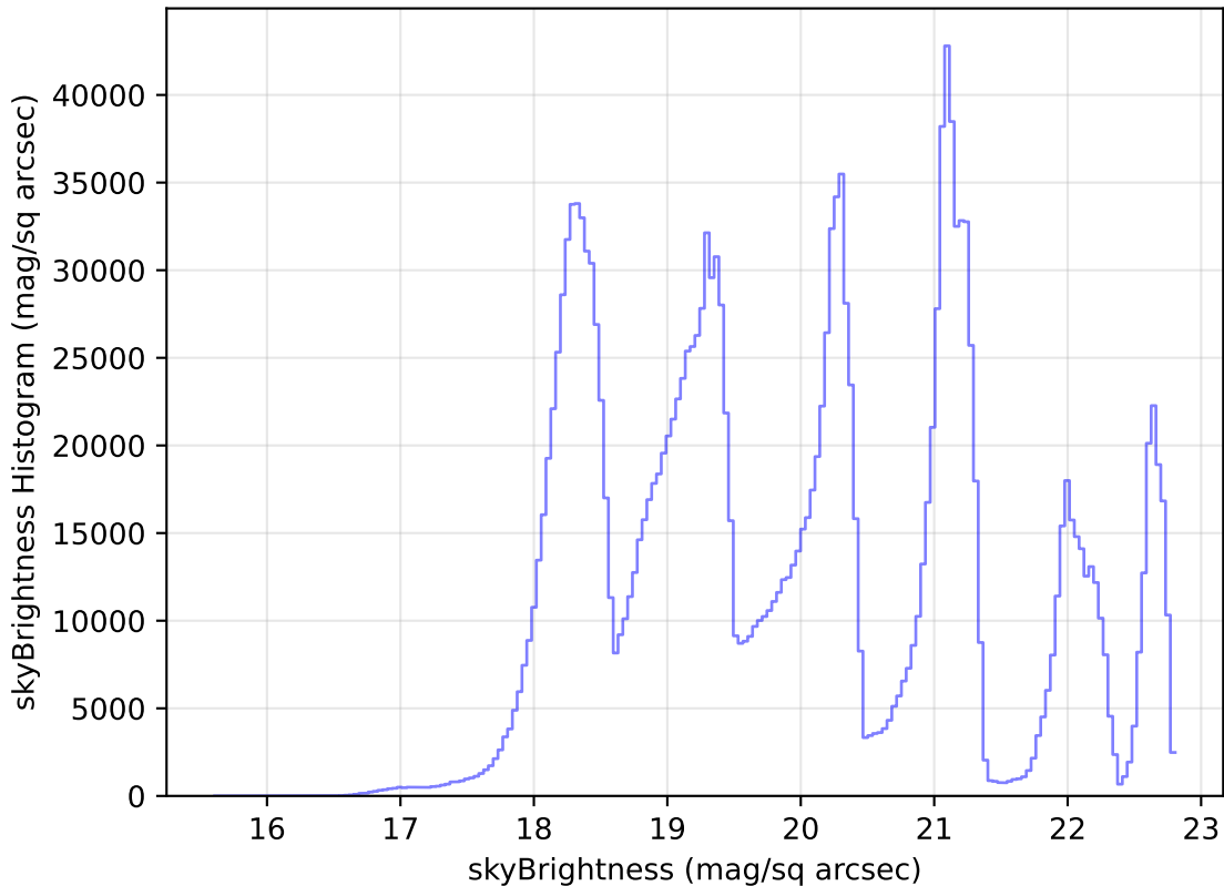
noroll_mjdp60_v3.4_10yrs WFD all bands: skyBrightness Histogram
