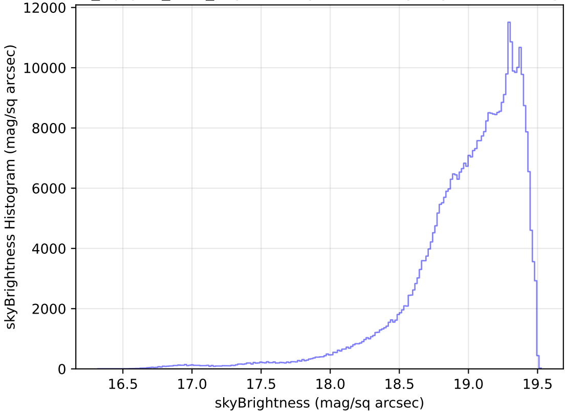
noroll_mjdp60_v3.4_10yrs All sky z band: skyBrightness Histogram
