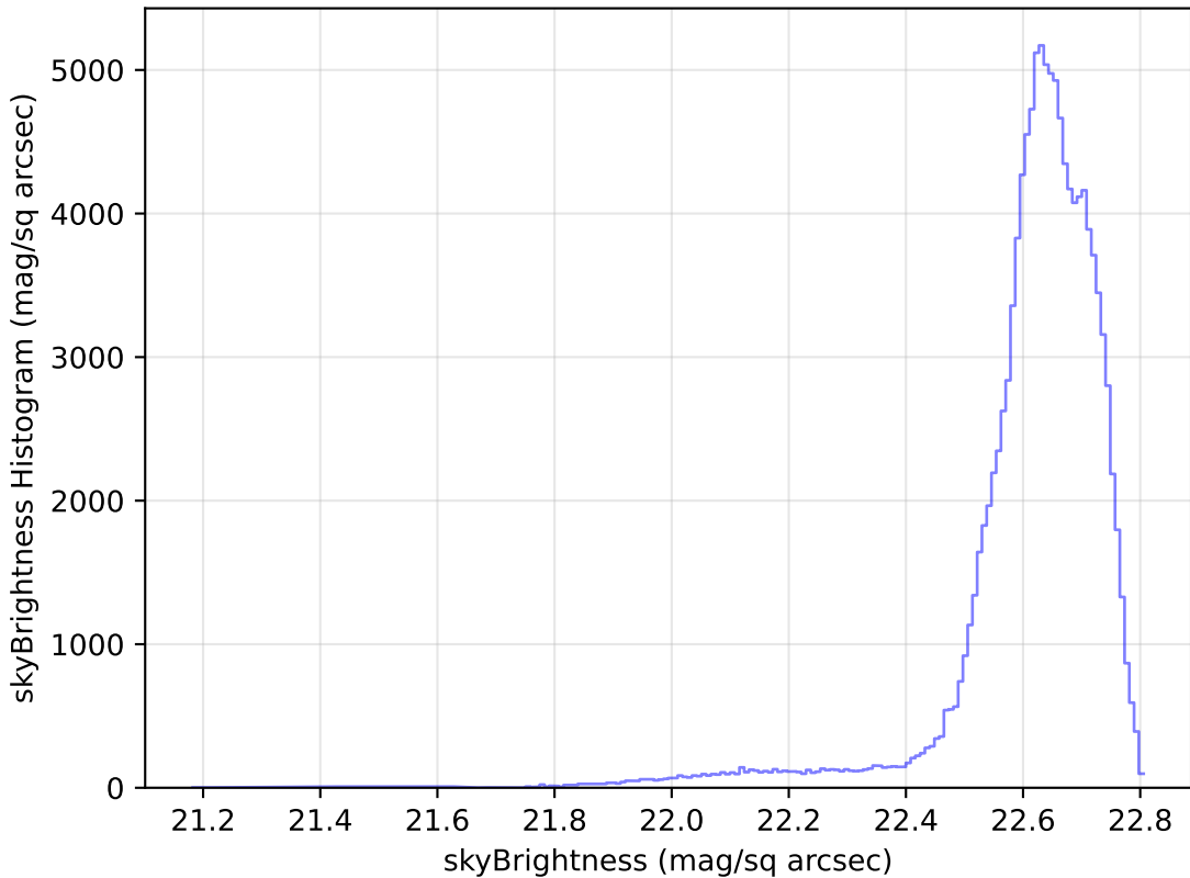
noroll_mjdp60_v3.4_10yrs All sky u band: skyBrightness Histogram
